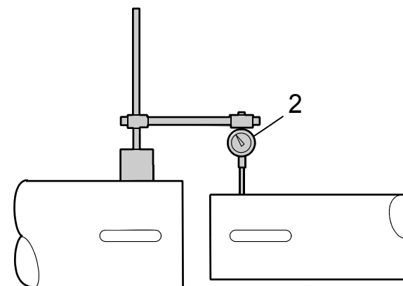
Measuring with free shaft ends.
