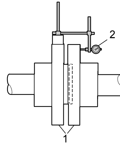
Measuring angular deviation.
