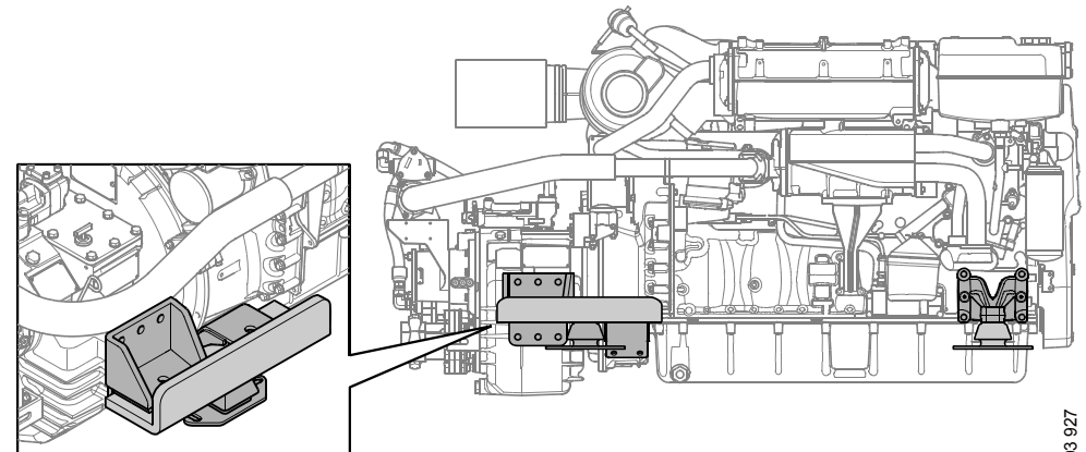
Example of four-point suspension with common rear bracket.
