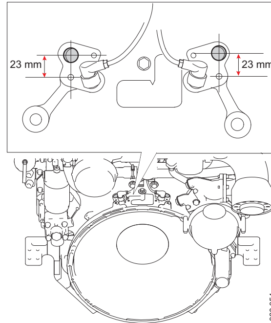
Connecting the rotational speed sensor, Ø 18 mm, 2 x M6 screws
