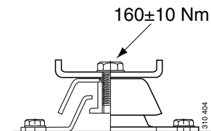
Tightening torque.
