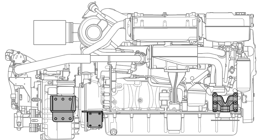
Example of six-point suspension.
